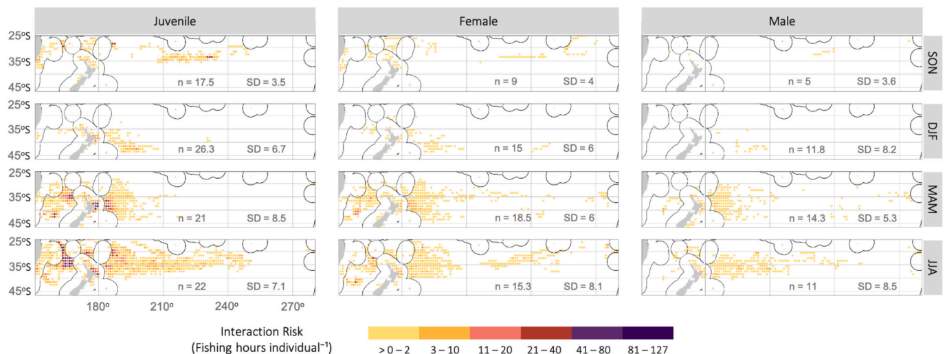
Fig. 3. Seasonal average interaction risk (IR), mean number of individuals (n) and standard deviation (SD) of Antipodean Albatross, grouped by sex and age (i.e., juvenile, female and male adult). Each 1° × 1° cell represents the mean of seasonal interaction risk (i.e., fishing hours individual -1 ) by the color gradient from yellow to dark purple (i.e., the dark shade indicates the higher IR) across the study period (2019–2022) within each austral season (i.e., spring – SON; summer – DJF; autumn – MAM; winter – JJA). (For interpretation of the references to color in this figure legend, the reader is referred to the web version of this article.)
