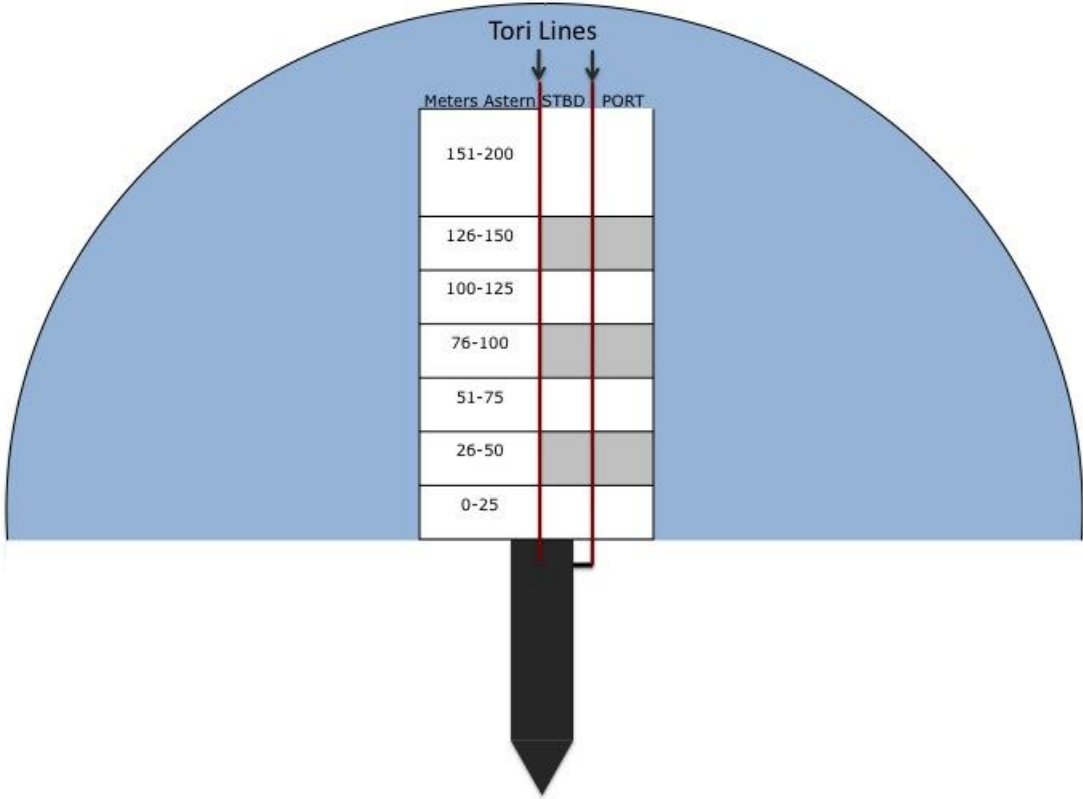
Figure 2. Distance bins (m) relative to starboard and port tori lines for attack rate data collection. Baited hooks were set on the port side between the wake and port tori line. Seabird abundance was estimated in a 250 m hemisphere centered at the stern during line setting and line hauling.
