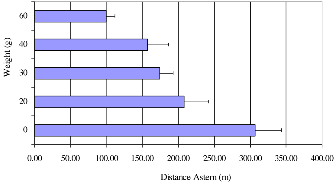
Figure 5. Estimated distance astern at which baited hooks sink to a benchmark depth of 10 m at a speed of 9.5 knots over ground. Error bars are 95% confidence intervals.
