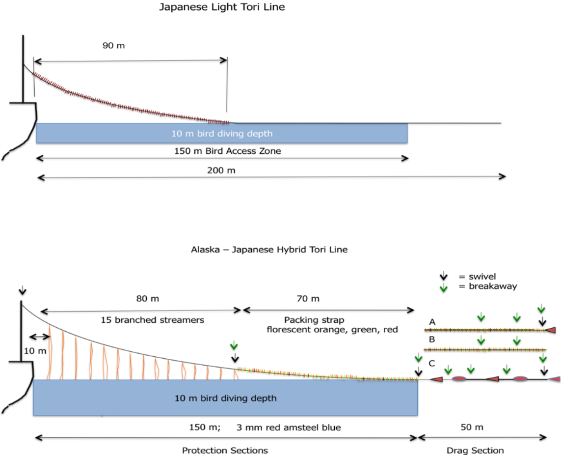
Figure 1. Schematics of tori lines. Light tori line (above) and hybrid tori line (bottom). Bird access zone is the distance astern baited hooks are above 10 m depth which was assumed to be 150 m for unweighted branchlines.
