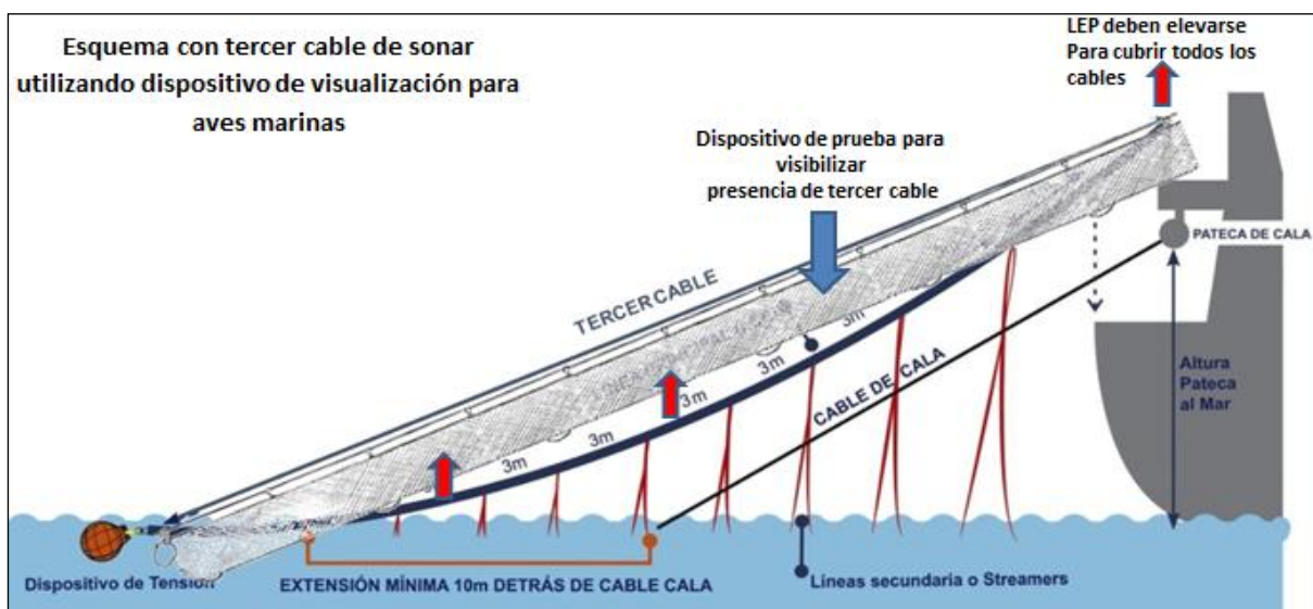
Figure 4. Schematic of a factory trawler using a third-wire cable curtain (Source: Subpesca, own elaboration).
