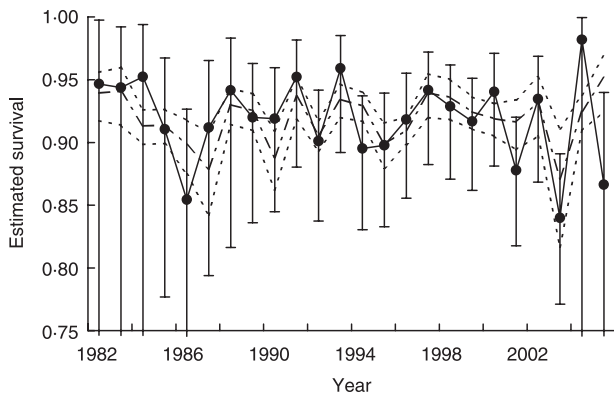
Fig. 4. Annual variations of adult survival probabilities estimated from the time-dependent model ( \Phi_t, p_{m+T+T^2+SSTA_{inc}} ) (●, solid line with error bars) and from the selected model ( \Phi_{LL_{winter}+SSTA_{inc}}, p_{m+T+T^2+SSTA_{inc}} ) (dashed lines with CI). Error bars, SE.
